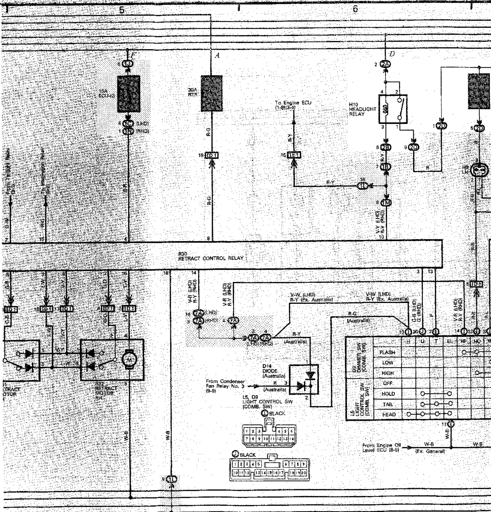
Headlight (Ex. Europe)
